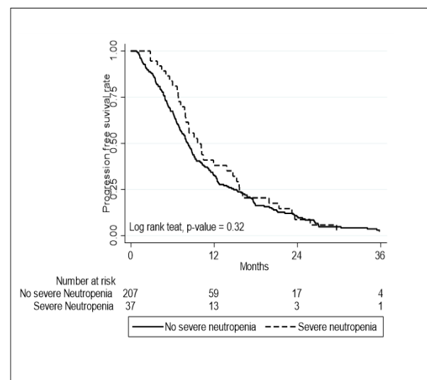
Figure 1. Progression-free Survival
