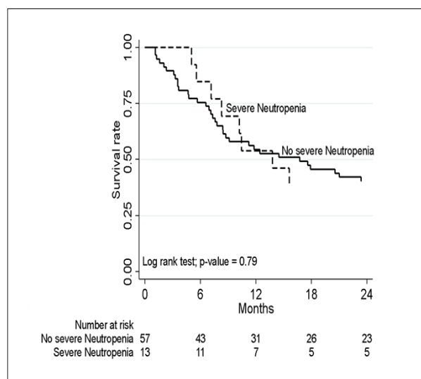
Figure 2. Overall Survival
