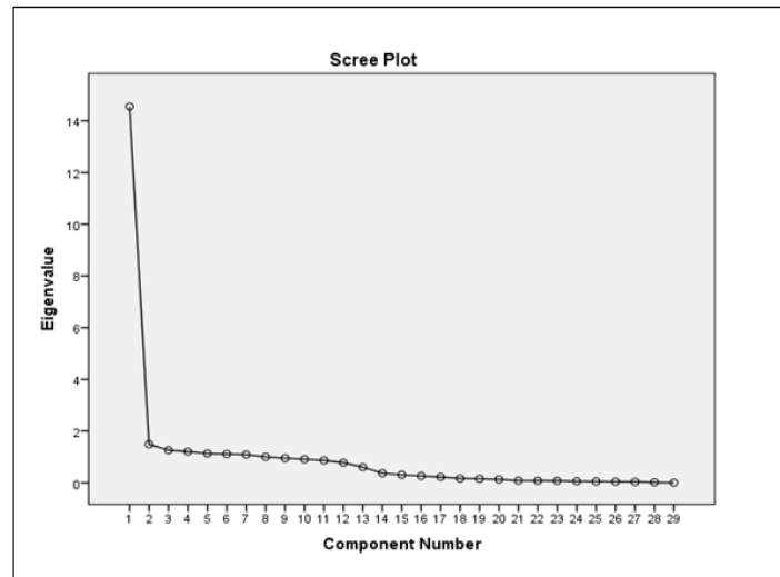
Figure 1. Scree Plot of Radiotherapy Administration Checklist
